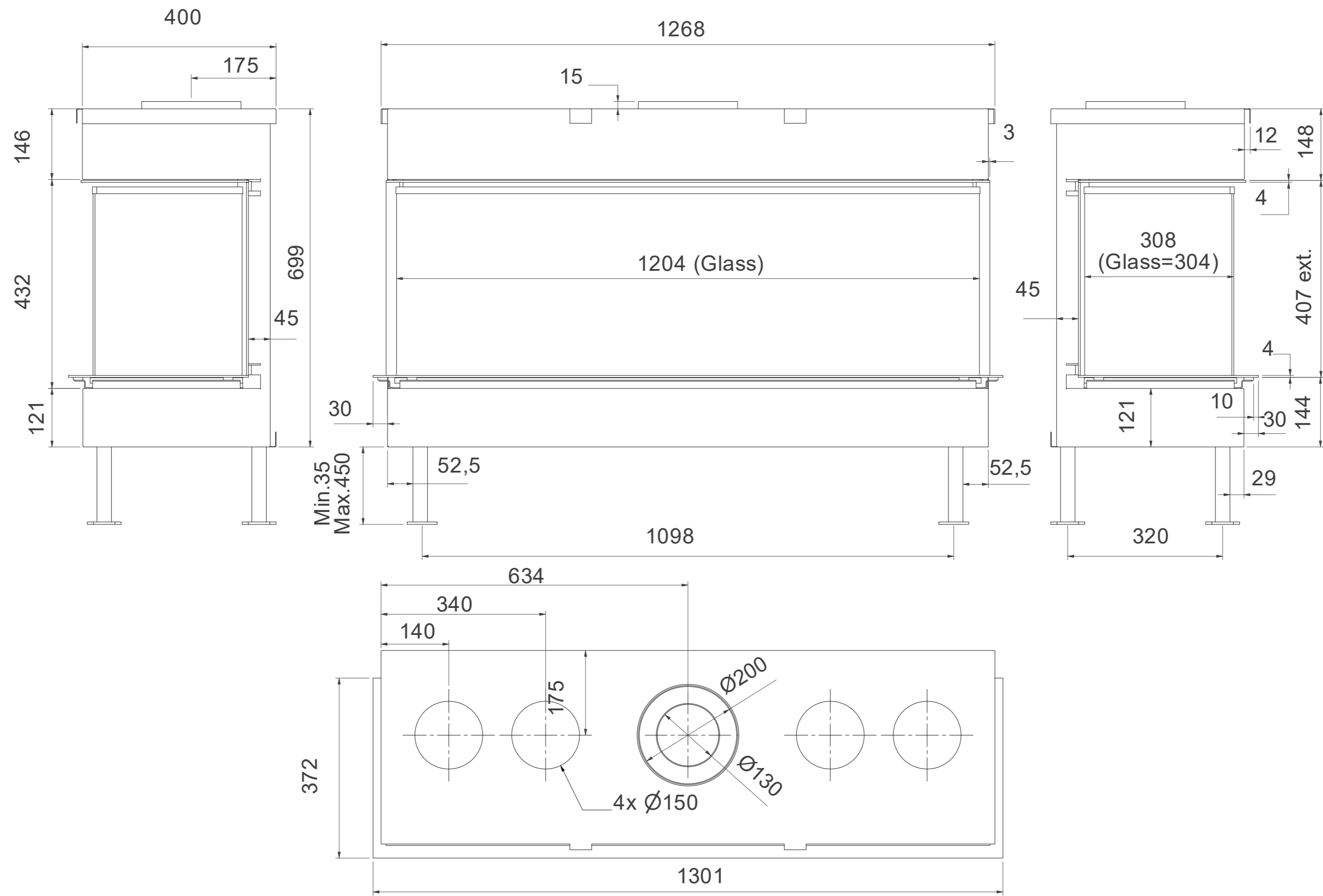
Luna Diamond 1300DC Gas/Gaz
