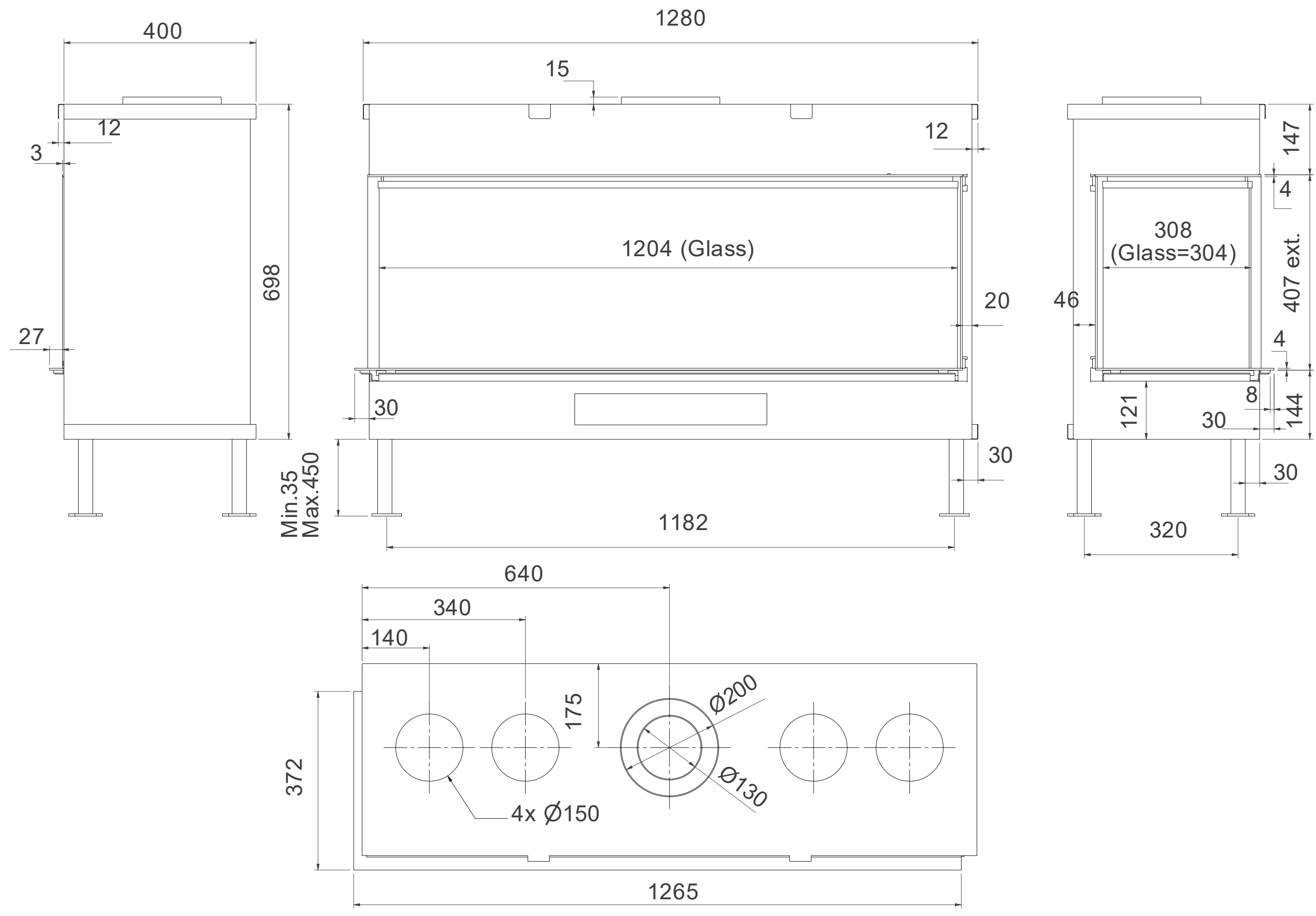
Luna Diamond 1300CL Gas/Gaz
